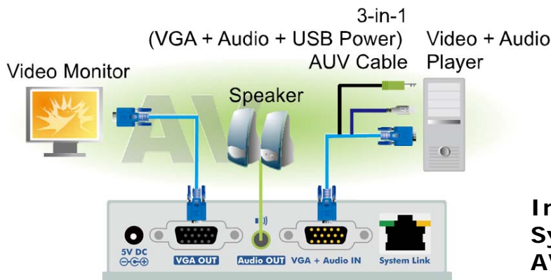
One Port Transmitter
